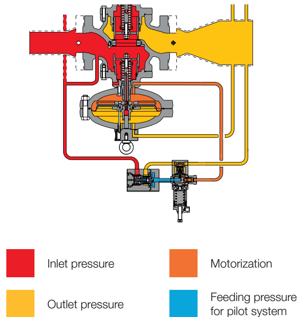
Figure 6 Reflux 819 with PM/819
